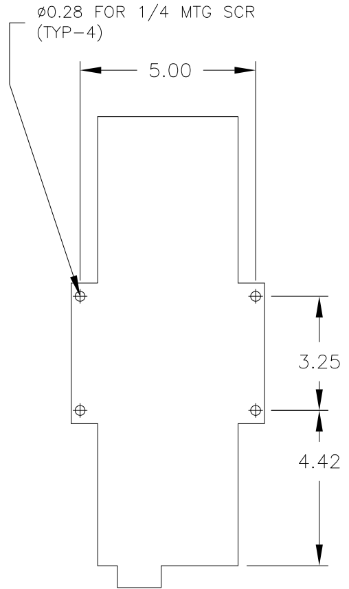
MOUNTING DIMENSIONS
