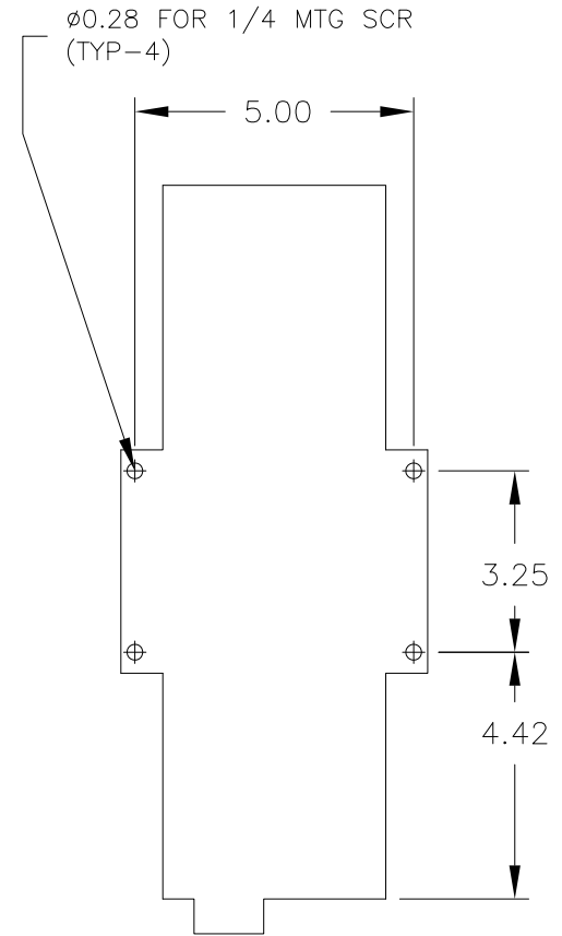
MOUNTING DIMENSIONS
